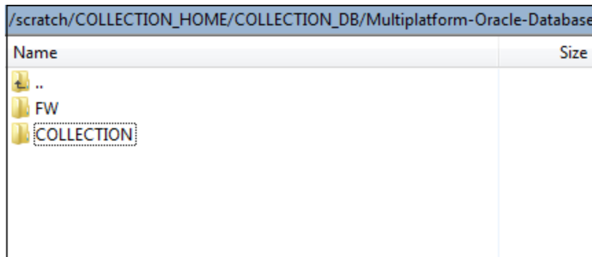
Figure 2–1 Extracted Multiplatform-Oracle-Database.zip
